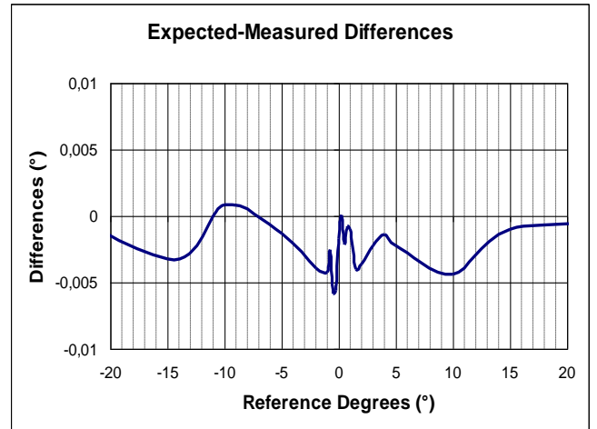
Figure 7. Difference between the measured values and expected values as a function of inclination angle ( x -axis).
