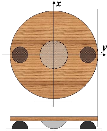
Figure 9: The constraints along y-axis allow to perform measurements of inclination angle only on x-axis.
